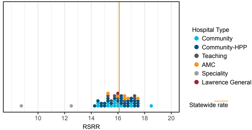
This graph shows the distribution of risk-standardized readmission rates for hospitals. Lawrence General Hospital is indicated by the red dot. Lawrence General Hospital is a hospital type of Community - High Public Payer. Please see the statewide report for more information on hospital type.
